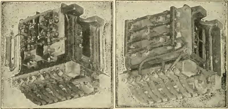
Fig. 63. Front and Back View of Sprague-General Electric Reverser
